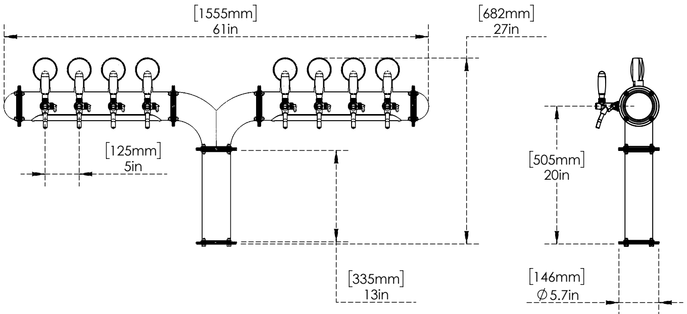
Front View
