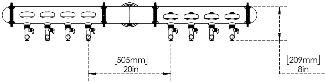
Top View
